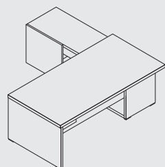
MIT1 2278 | 2080 | 740 89 3/4" | 82" | 29 1/8"
